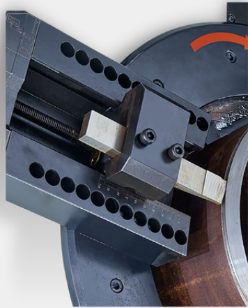
STANDARD TOOL POST
