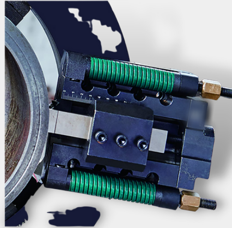
OD TRACKING ATTACHMENT
